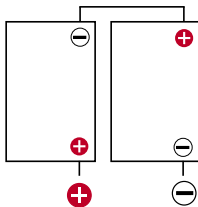
SERIES CONNECTION
